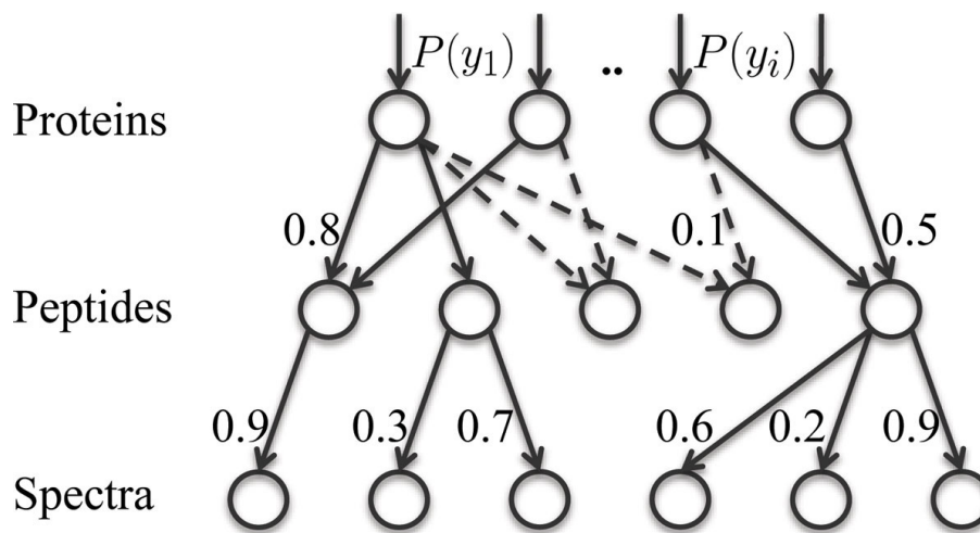
Figure 5 An example of a Bayesian network used as a generative model in MSBayesPro. Three layers are provided reflecting the LC-MS/MS experiment in which proteins are first digested into peptides which are then matched to the MS/MS spectra. The numbers associated with the directed edges indicate peptide detectabilities (between the first two layers) and PSM identification scores (between the last two layers). Note that some peptides may not be matched with any spectra while some others may be matched with more than one spectrum. The peptides not matched to any spectra are shown using dashed lines.
