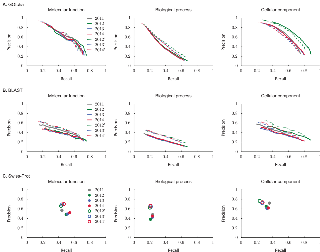
Fig. 6. Precision-recall evaluation on each GO classification using (A) Götcha, (B) BLAST and (C) Swiss-Prot predictions from January 2010. Solid gray curves (filled circles) represent performance of each method using proteins that did not have experimental annotation in 2010 but were experimentally annotated in January 2011. Color curves show evaluation on those proteins from the 2011 set that accumulated new annotations in 2012 (green), 2013 (blue) and 2014 (red). Solid curves (filled circles) show incomplete-data evaluation on each subset of proteins, whereas dotted curves (empty circles) show complete-data evaluation
