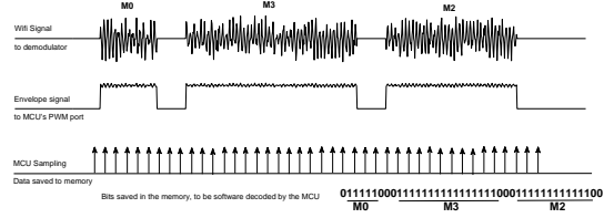
Fig. 3. PWM decoding.
