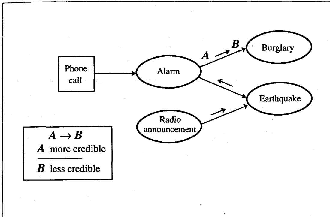
Figure 1.2. Making the antecedent of a rule more credible can cause the consequent to become less credible.
