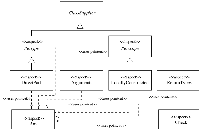
Figure 3: The UML diagram of the class form checker
