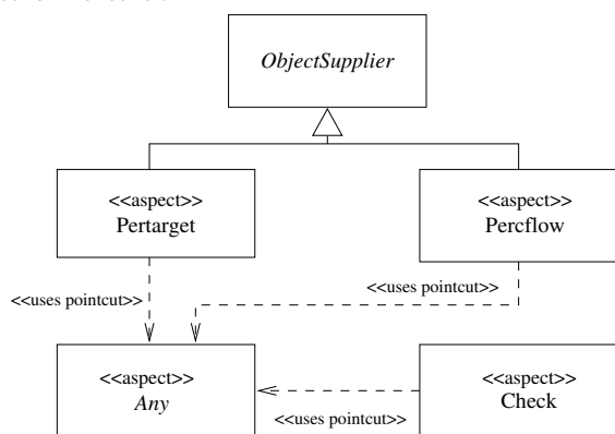
Figure 2: The UML diagram of the object form checker
