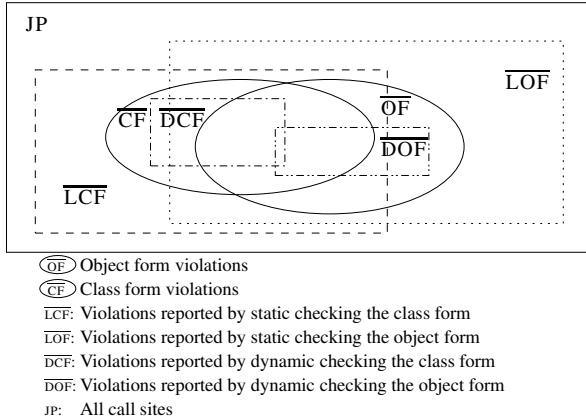
Figure 1: The relationship between different LoD predicates.
