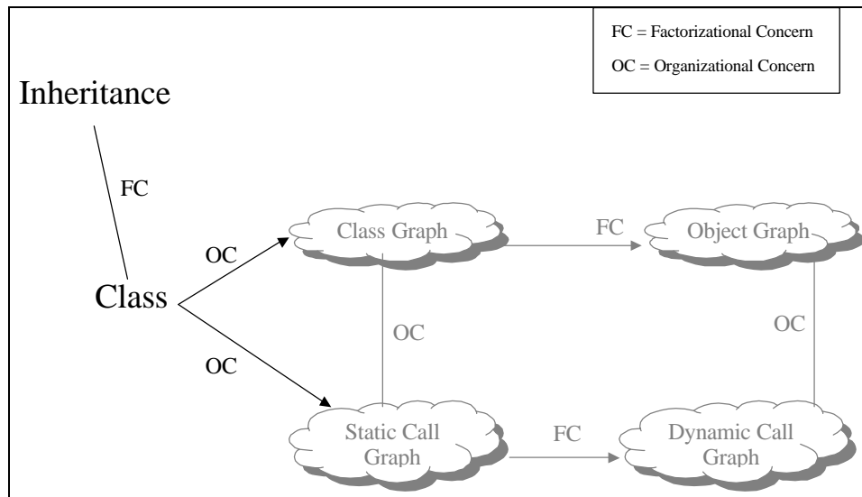
Figure 69: Concern Relationship Diagram for OOP Features Class and Inheritance
