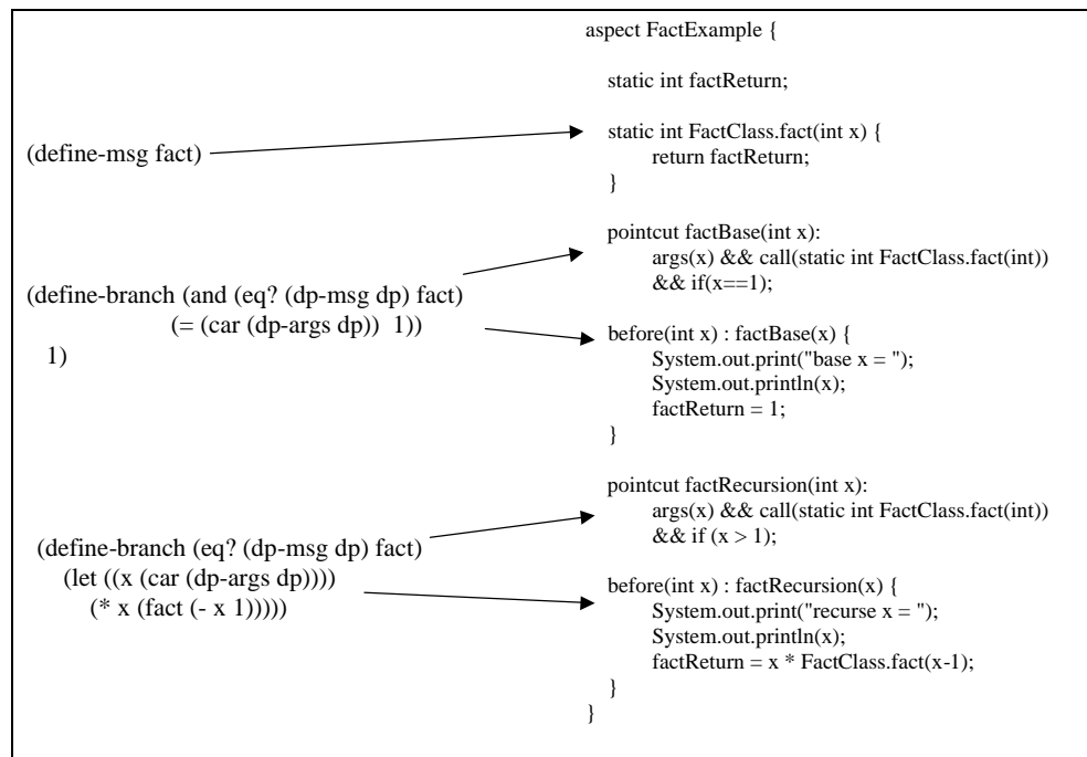
Figure 31: Factorial Example Translated from Fred to AspectJ
