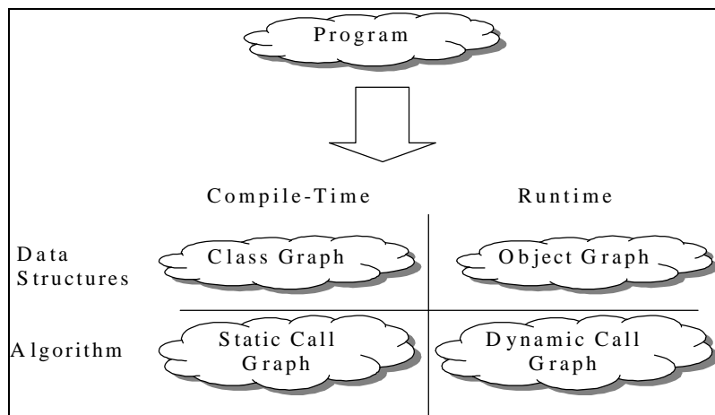
Figure 62: Graphic Decomposition of Programs
