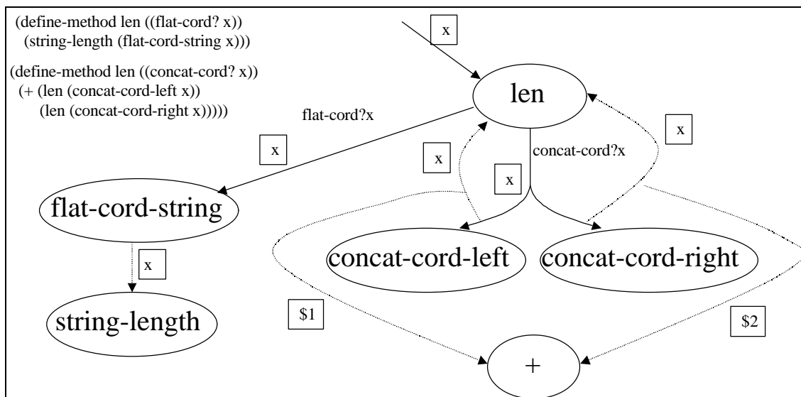
Figure 29: Graphical Notation for len
