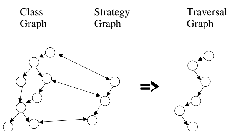
Figure 78: Visualization of the Relationship between Class Graph, Strategy Graph and Traversal Graph
