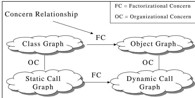
Figure 68: Concern Relationship Diagram of 4GMP
