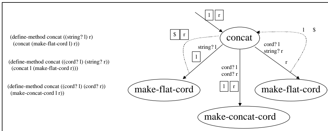
Figure 28: Graphical Notation for concat
