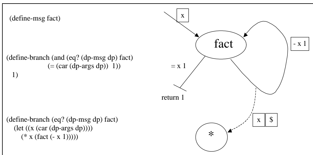
Figure 27: Graphical Translation of Factorial Example
