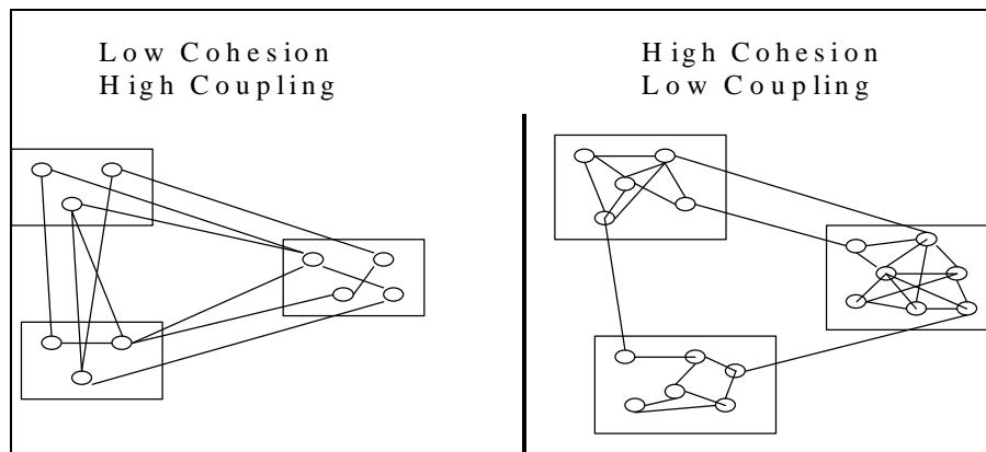
Figure 67 Cohesion and Coupling from [8 Tucker 1997]
