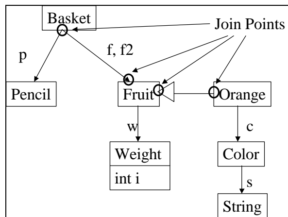
Figure 40: Join points for the Basket Example Class Graph
