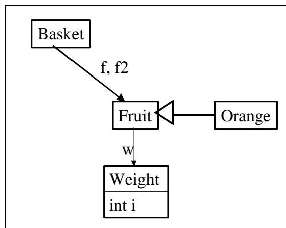
Figure 11: Traversal Graph as a result of applying the Strategy "from Basket to Weight" to the Basket Example Class Graph
