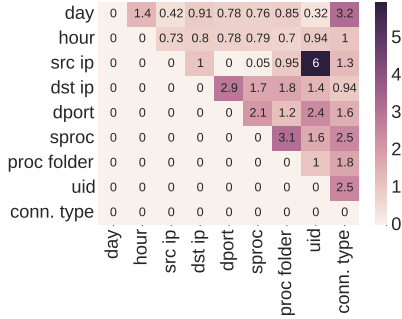
Figure 5: Pairwise weights learned for P2I events.
