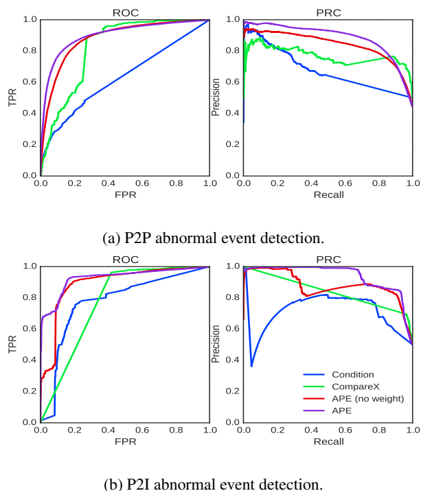
Figure 3: Receiver operating characteristic curves and precision recall curves for abnormal event detections.
