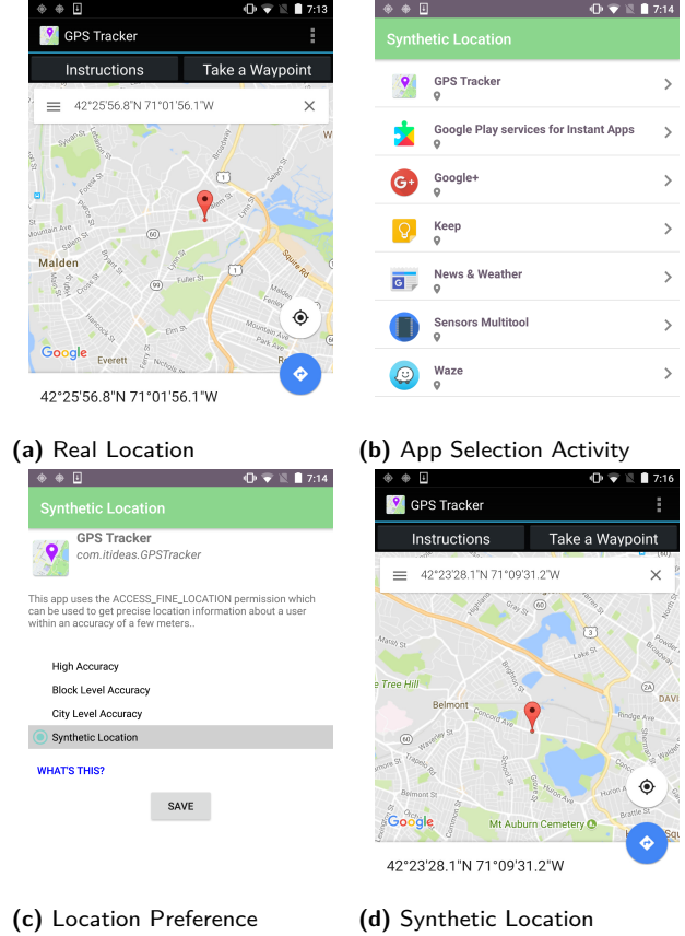
Fig. 5. Example screenshots of the Synthetic Location GUI.
