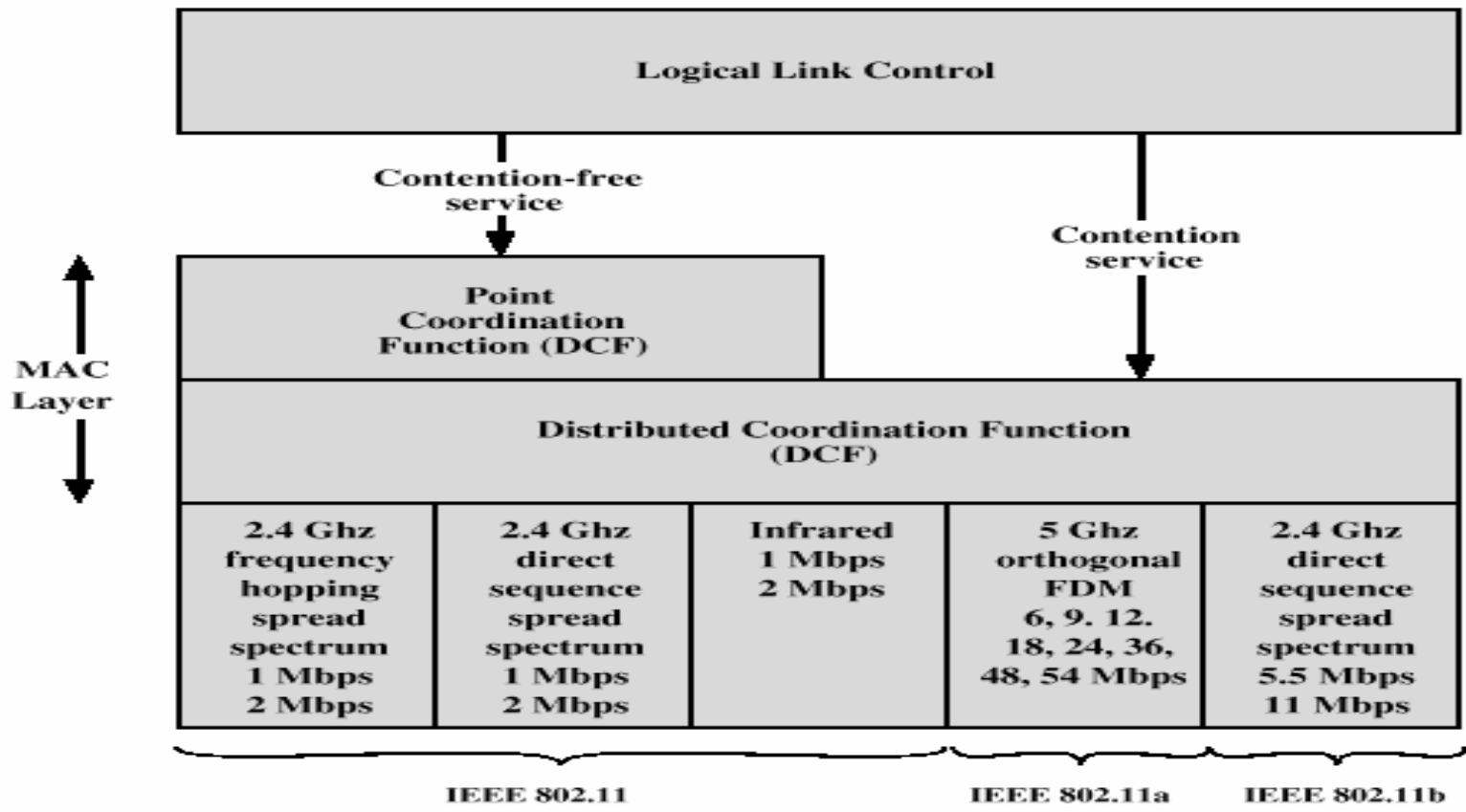
Figure 14.5 IEEE 802.11 Protocol Architecture
