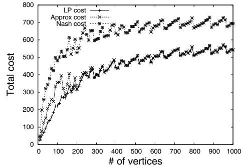
Fig. 7. The costs of the LP solution, our approximation algorithm, and the Nash equilibrium computed by best response, for the local model in random geometric graphs.
