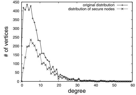
Fig. 6. Properties of secured nodes in NE in power law graphs.
