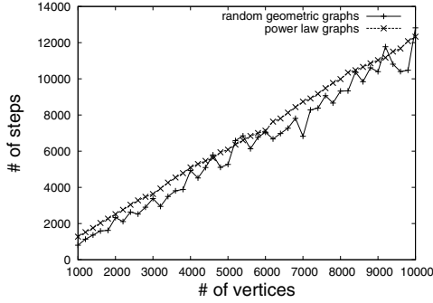
Fig. 4. Convergence time in the global model ( d = \infty ) for random geometric graphs and power law graphs.
