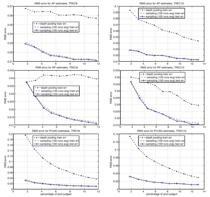
Figure 12: RMS error train/test comparisons for MAP, RP, PC(30), in TREC8 and 10. Equivalent depths are indicated on the plot.
