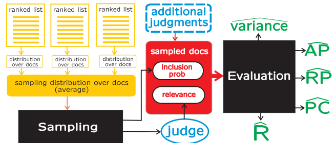
Figure 3: Sampling and evaluation design
