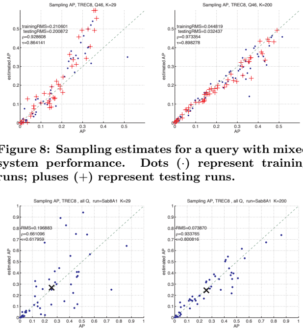
Figure 9: Sampling estimates for a fixed typical run (Sab8A1) with MAP = 0.25, all queries. Each dot ( \cdot ) is an AP for a query estimate (total 50); MAP estimate is plotted as “ \times ”.
