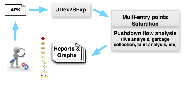
Figure 4. Software Architecture
