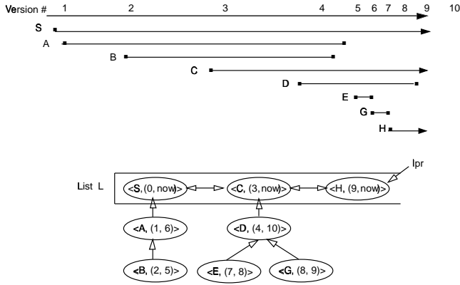
Figure 3. Snapshot Index.
