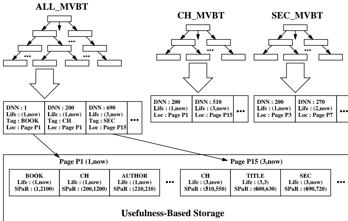
Figure 5. Index organization.
