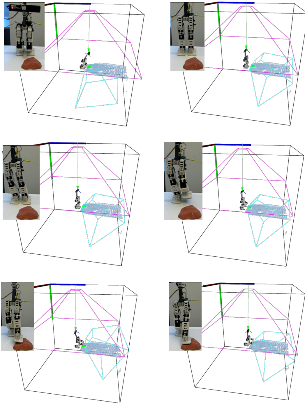
Figure 59: RPBP detecting a patch on rock 1 for foot placement and proceeding with the predefined motion (Figure 58, first row). The TDSF volume outline appears with the robot, the point cloud, the physical and virtual overhead camera frusta, and the patch at each step.
