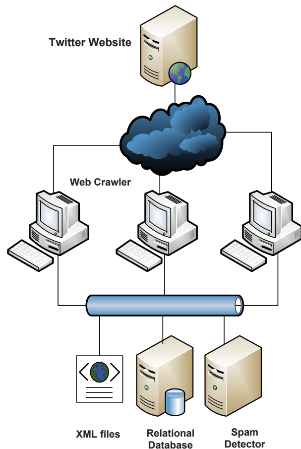
Figure 5: Twitter Spam Detection System
