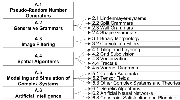
Fig. 2. Taxonomy of common methods for generation game content. The label in each box (such as “A.1” in the “Pseudo-Random Number Generator” box, at the top) refers for each method to its section in Appendix A.
